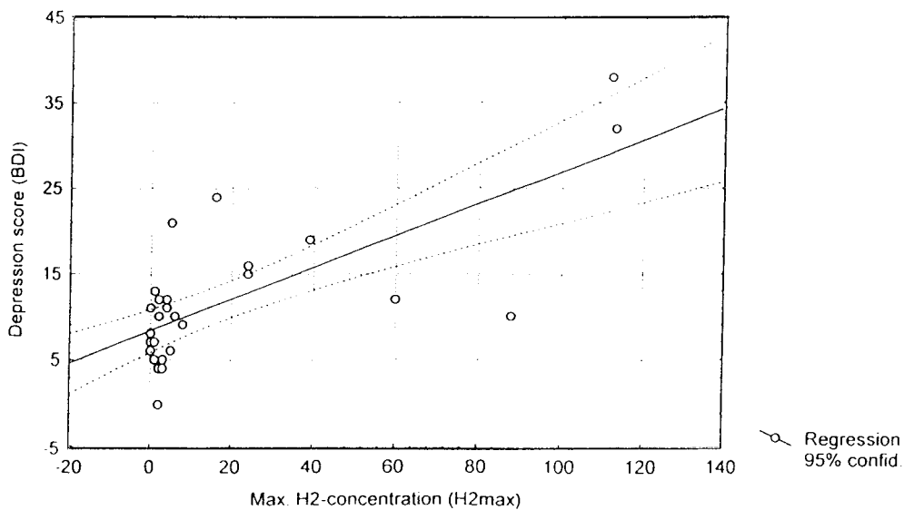
Fig 2. Depression score vs max H_2 concentration. BDI = 8.3404 + 0.18604 \cdot H_2max . Correlation: r = 0.72772 ; P < 0.05 .
